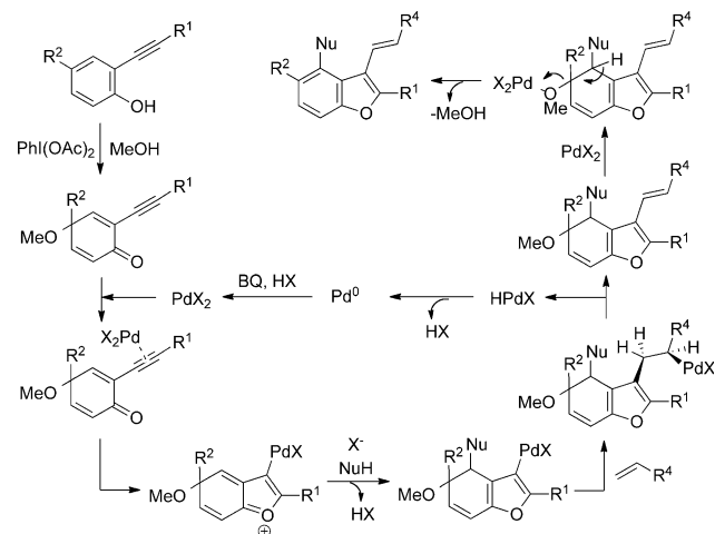
Scheme 2. Plausible mechanism.
