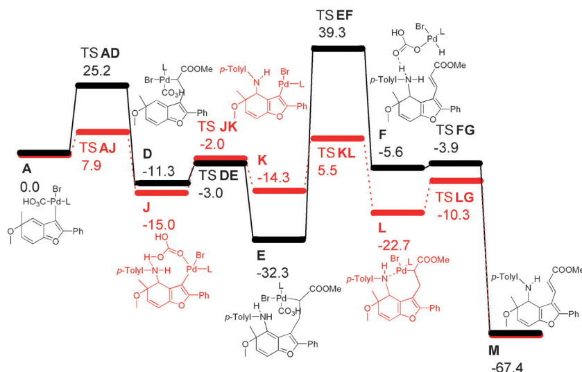
Figure 2. Free-energy reaction profile (kcal mol -1 ) from intermediate A to the non-aromatized product, calculated at the PCM(DCE) B3LYP/6-31G(d,p) with LANL2DZ (for Pd and Br) level. TS = transition state.
